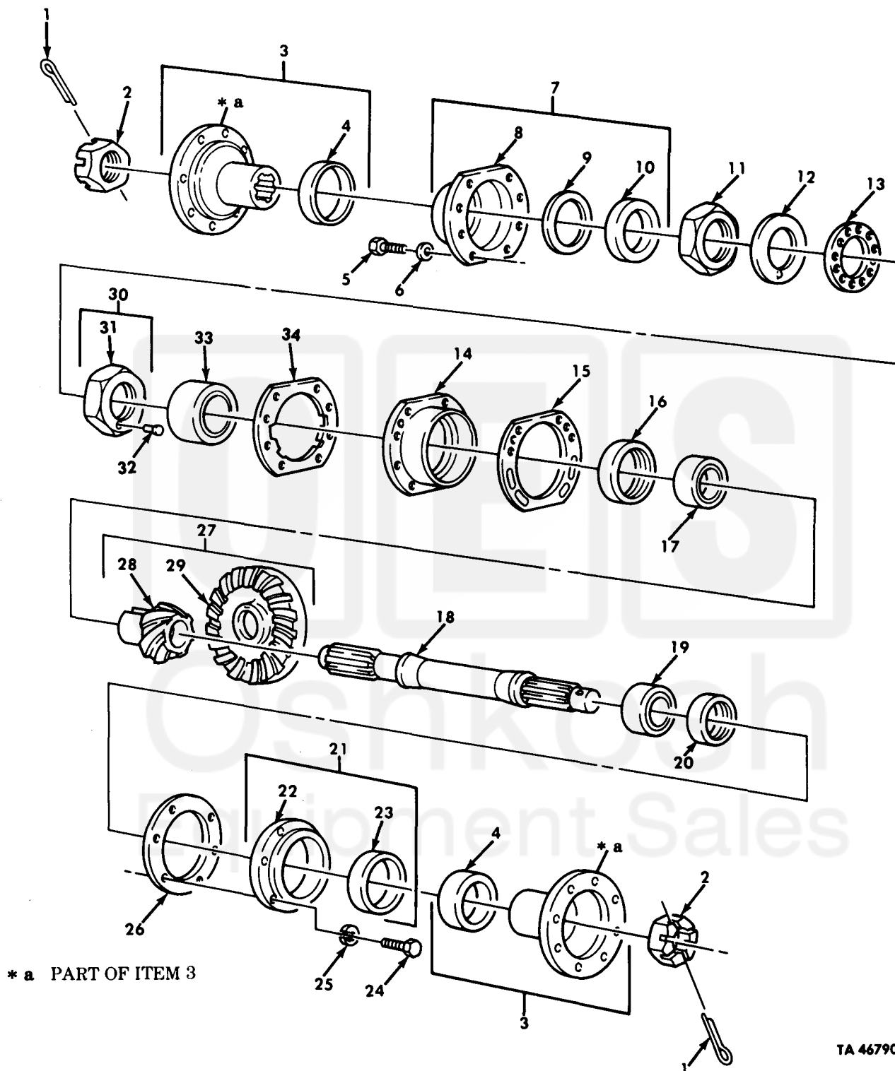
Figure 170. Front Axle Differential Through Shaft, Gears, and Flange Assemblies.
